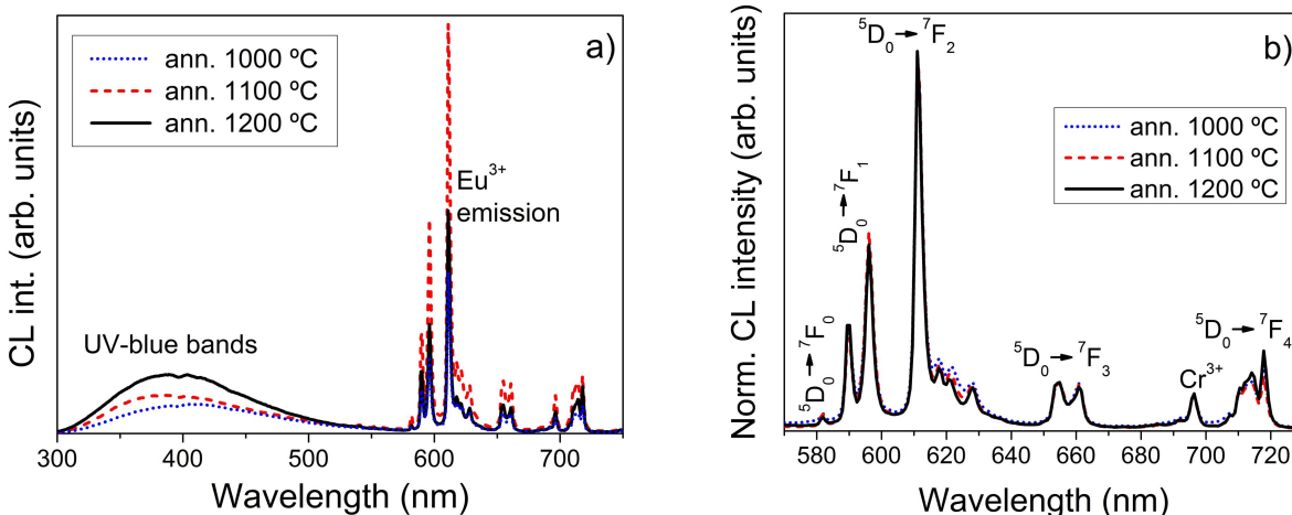
Figure 5. (a) RT CL spectra ( V_{acc}=5 kV) of \text{Ga}_2\text{O}_3 bulk samples implanted with 4 \times 10^{15} \text{at}/\text{cm}^2 and subjected to RTA up to 1200^\circ\text{C} . (b) Normalized CL spectra, showing the wavelength region of the {}^5\text{D}_0 \rightarrow {}^7\text{F}_j intraionic \text{Eu}^{3+} transitions.
